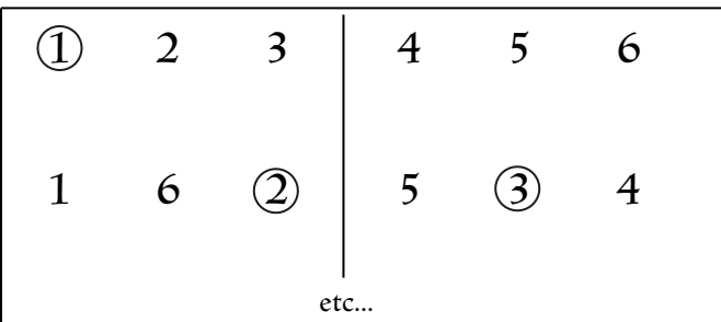
Oscil permutation pattern
